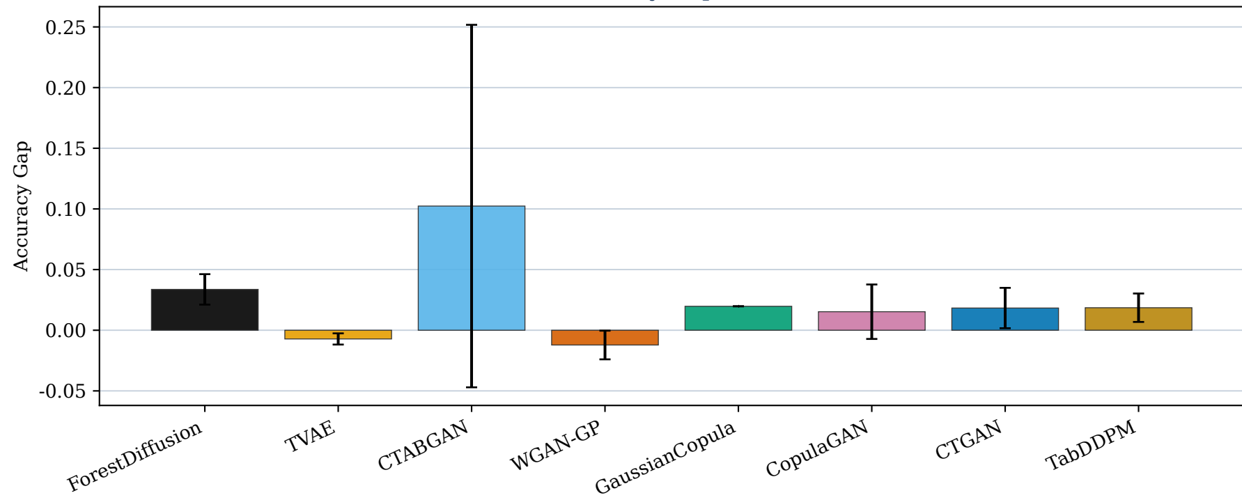
CDC Diabetes — Accuracy Gap (mean \pm SD, 10 seeds)
